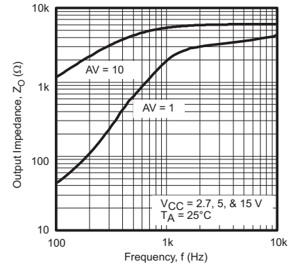
Figure 18. Output Impedance vs Frequency
