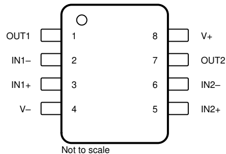
TLV2402-Q1 DGK Package 8-Pin VSSOP Top View
