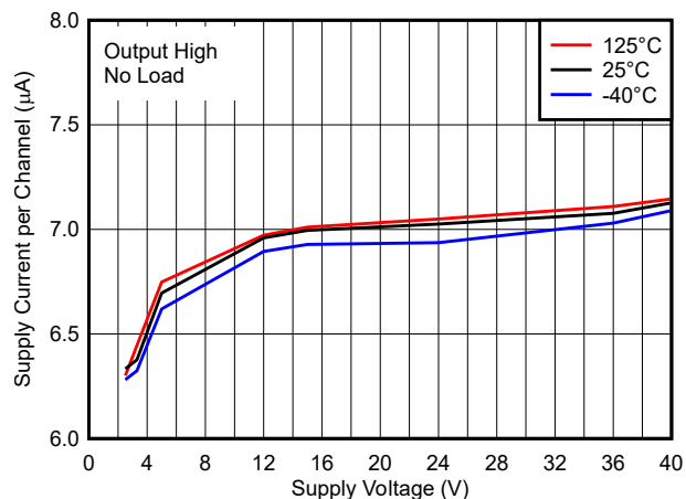
TLV18xx-Q1 Supply Current vs. Supply Voltage
