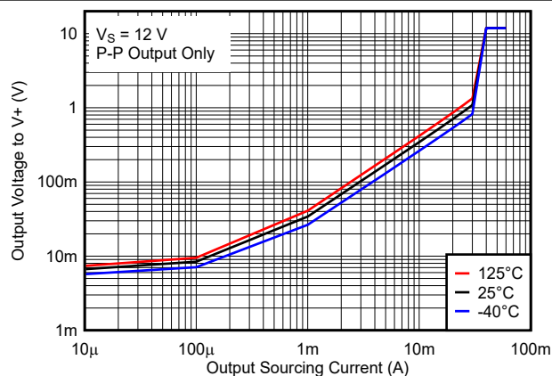
Figure 6-8. Output Voltage vs. Output Sourcing Current, 12V
