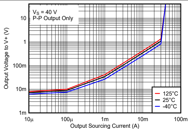
Figure 6-10. Output Voltage vs. Output Sourcing Current, 40V
