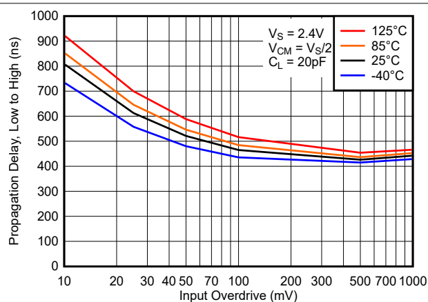
Figure 6-12. Propagation Delay, Low to High, 2.4V
