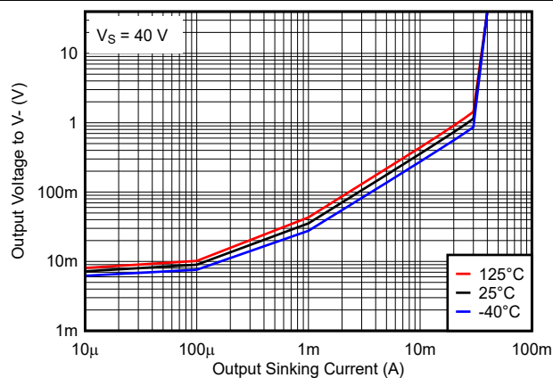
Figure 6-9. Output Voltage vs. Output Sinking Current, 40V
