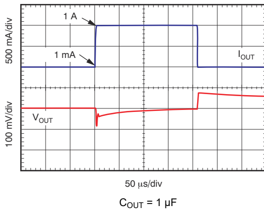
Figure 6-19. Load Transient Response 1 mA to 1 A
