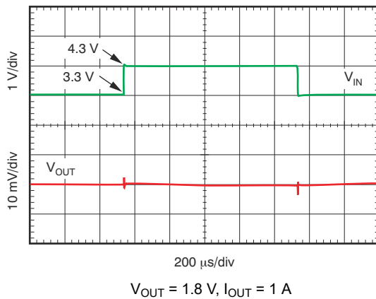
Figure 6-23. Line Transient Response
