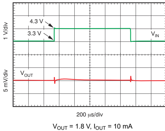
Figure 6-21. Line Transient Response
