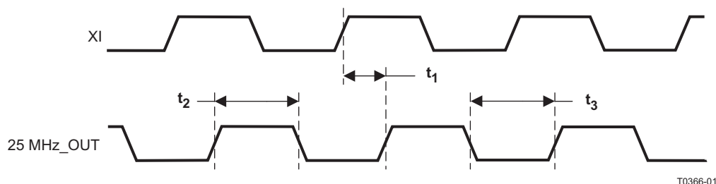
Figure 9-24. 25 MHz_OUT Timing
