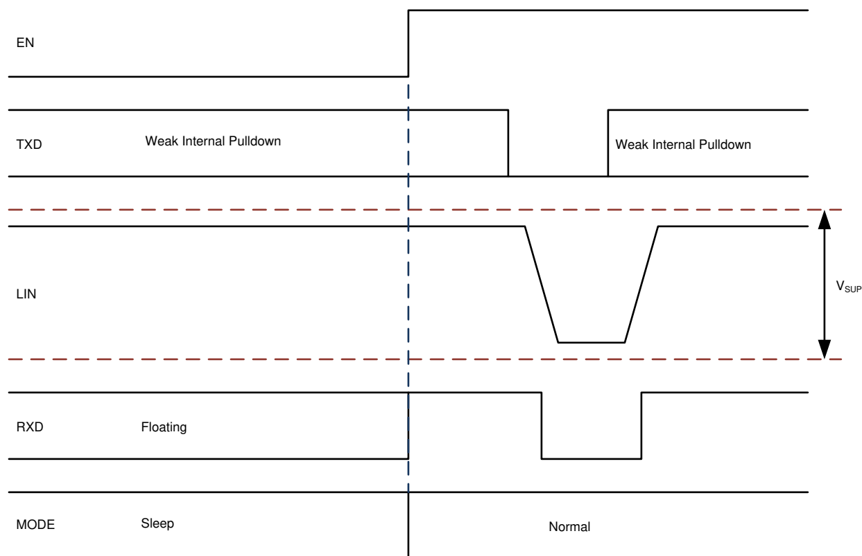
Figure 8-14. Mode Transitions
