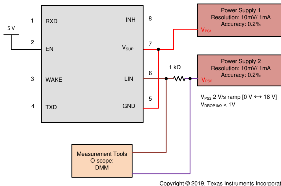
Figure 8-9. Test Circuit for I_{BUS\_NO\_GND} Loss of GND
