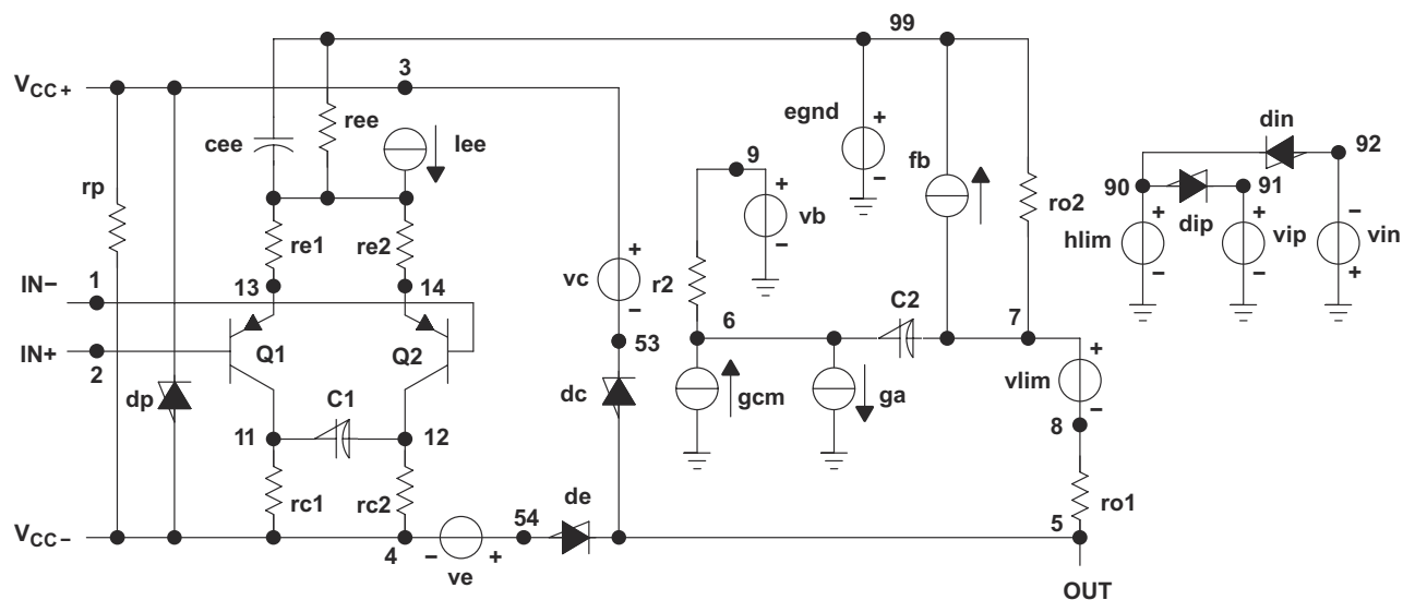
Figure 8-3. Boyle Subcircuit
