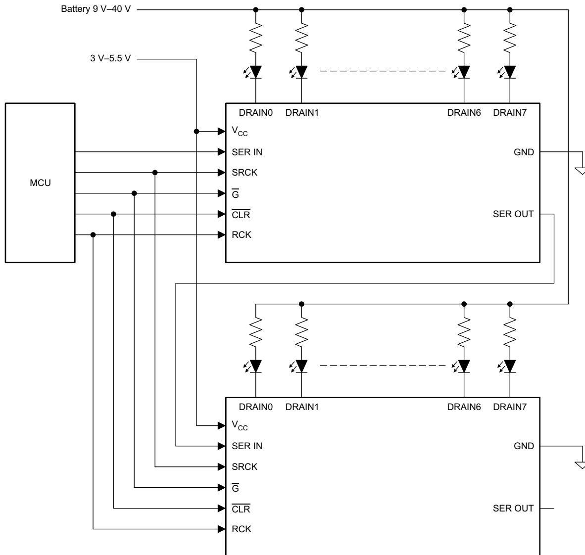
Figure 14. Typical Application Circuit
