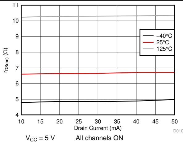
Figure 9. r_{DS(on)} vs Drain Current
