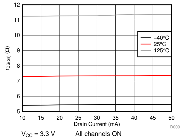
Figure 8. r_{DS(on)} vs Drain Current
