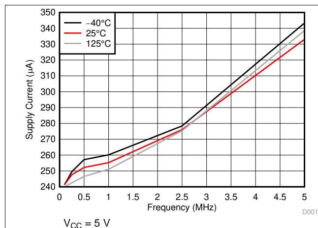
Figure 3. Supply Current vs CLK Frequency
