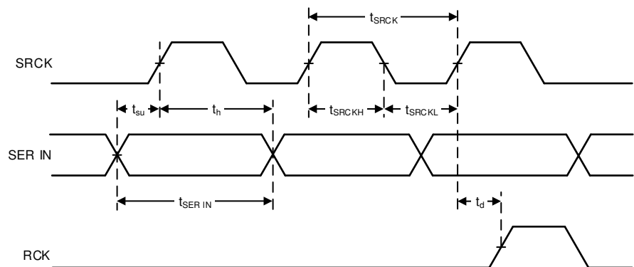
Figure 1. Timing Diagram of Input Signals
