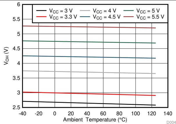
Figure 11. SER OUT High Voltage vs Temperature (°C)
