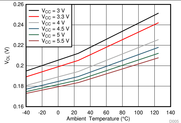
Figure 12. SER OUT Low Voltage vs Temperature (°C)
