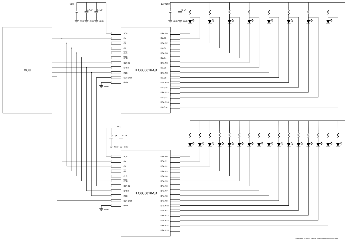
Figure 20. Typical Application Circuit
