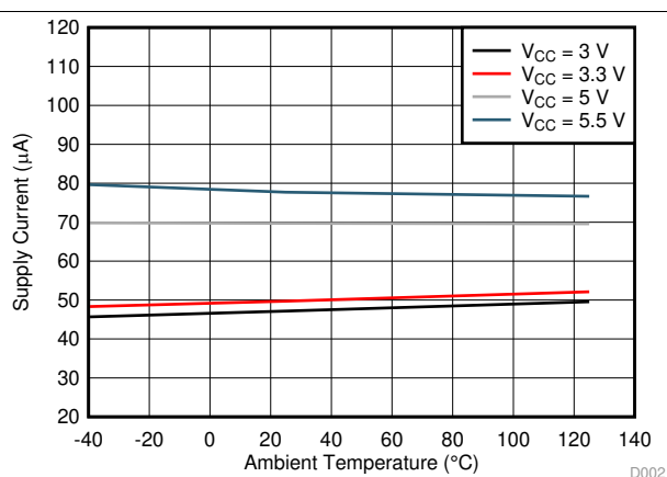
Figure 4. Supply Current vs Ambient Temperature
