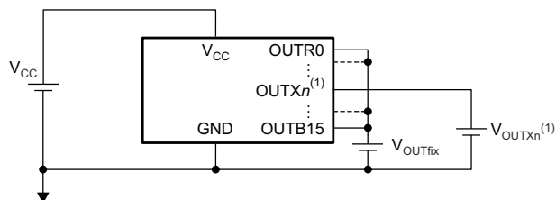
Figure 7-6. Constant-Current Test Circuit for OUTXn
