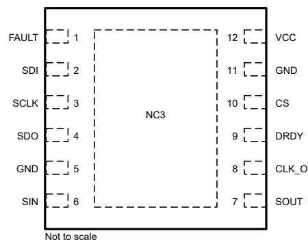
Figure 5-2. TLC6989 DRR Package 12-pin WSO with Exposed Thermal Pad Top View
