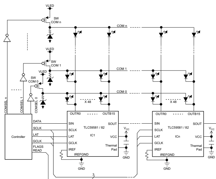
Typical Application Schematic (Multiple Daisy-Chaind TLC59581/82)
