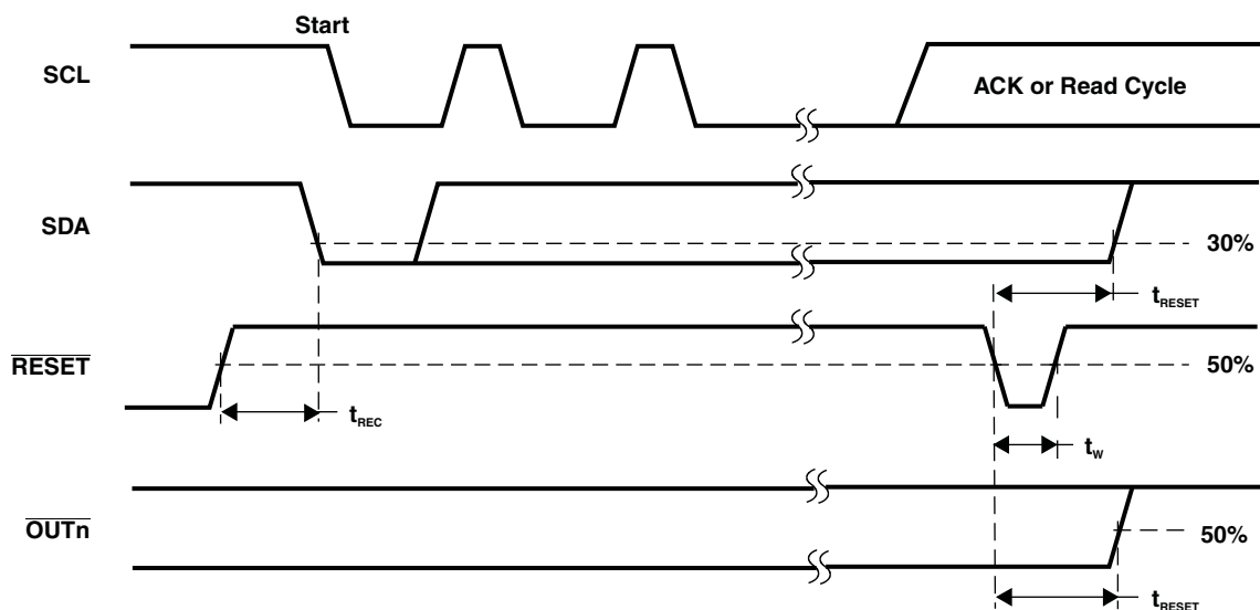
Figure 3. Reset Timing
