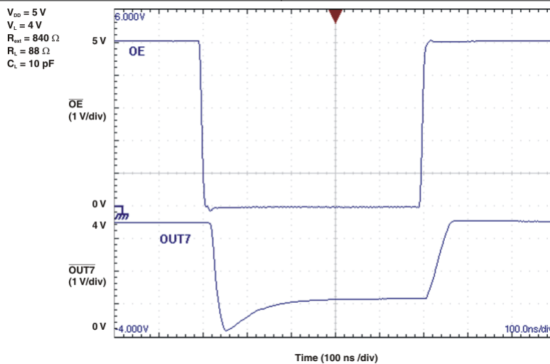
Figure 6-4. \overline{\text{OE}} to \overline{\text{OUT7}}
