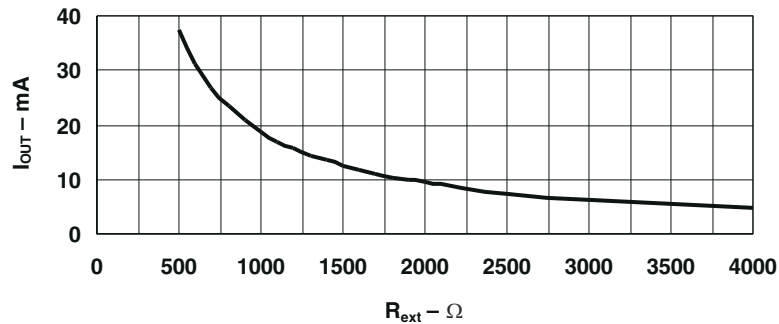
Figure 9-3. Default Relationship Curve Between I_{OUT,target} and R_{ext} After Power Up
