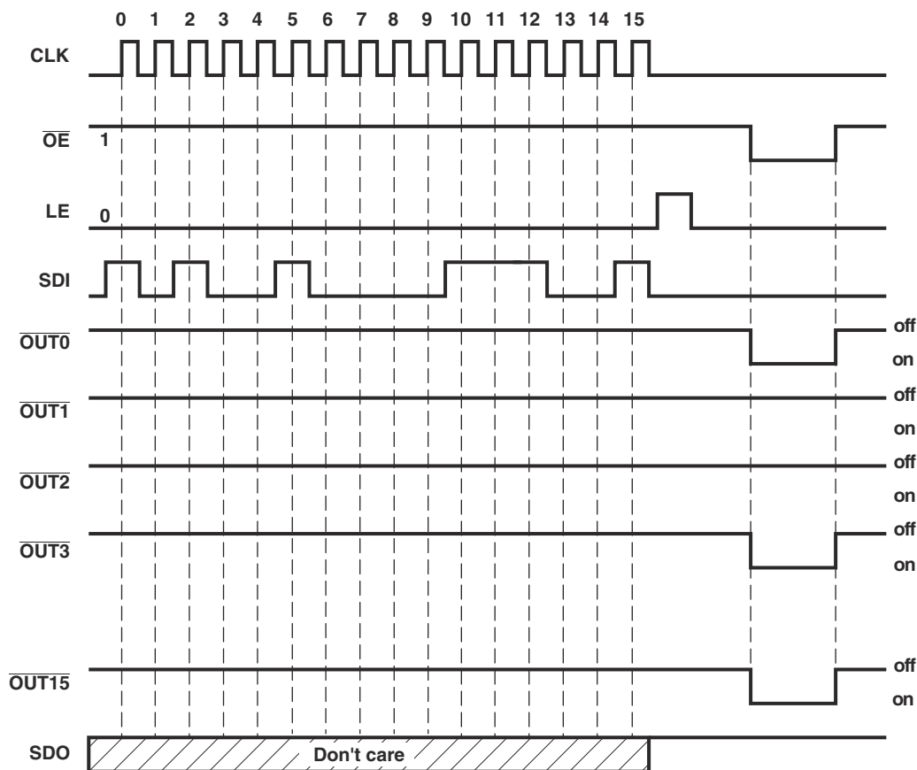
Figure 6-1. Timing Diagram
