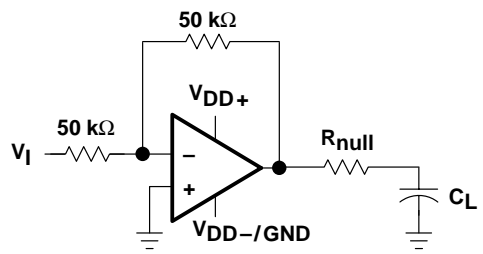
Figure 60. Series-Resistance Circuit
