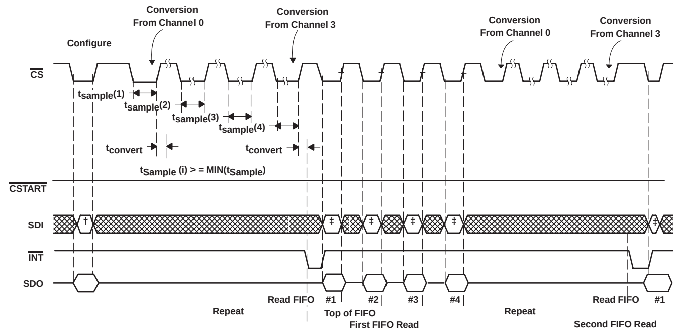
Figure 14. TLC1514/TLC1518 Mode 10/11 \mu p Serial Interface (conversions triggered by \overline{\text{CS}} )
