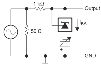
Figure 6-8. Test Circuit for Reference Impedance
