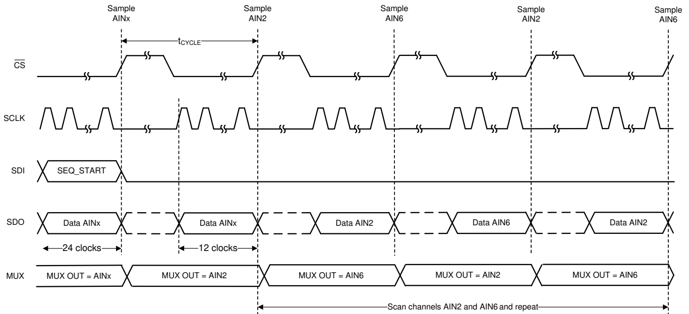
Figure 33. Starting Conversions and Reading Data in Auto-Sequence Mode
