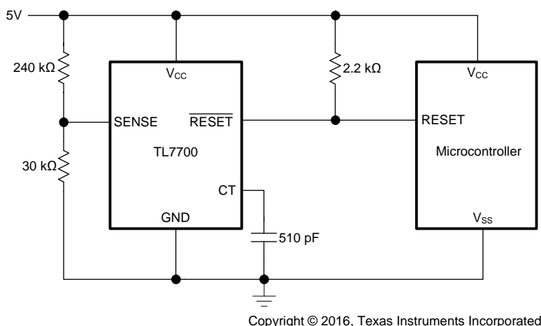
Figure 21. 5-V Supply Voltage Supervision
