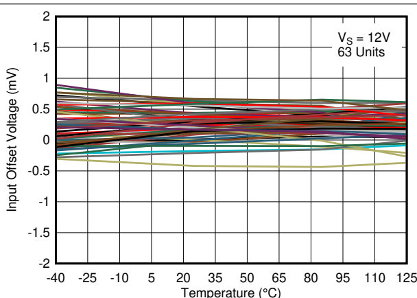
Figure 5-17. Input Offset Voltage vs. Temperature at 12V
