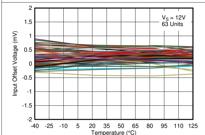
Figure 5-17. Input Offset Voltage vs. Temperature at 12V
