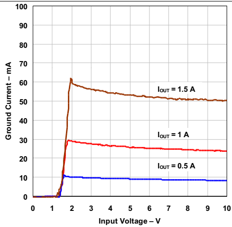
Figure 9. Ground Current vs Input Voltage
