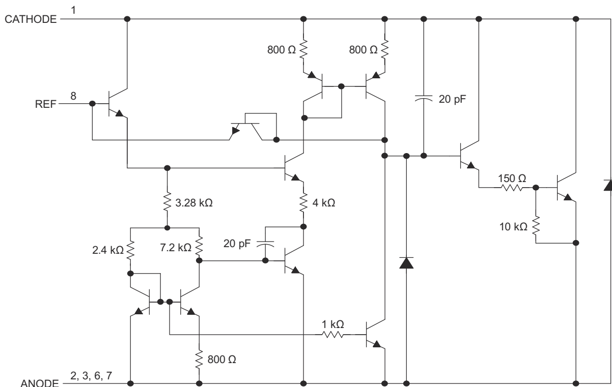
Figure 8-2. Equivalent Schematic
