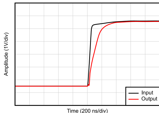
Figure 5-31. Small-Signal Step Response, Rising
