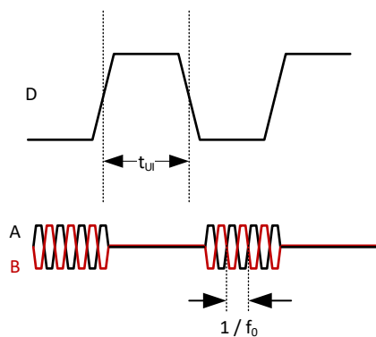
Figure 7-3. Measurement of Carrier Frequency
