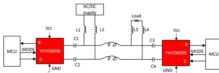
Simplified Schematic
