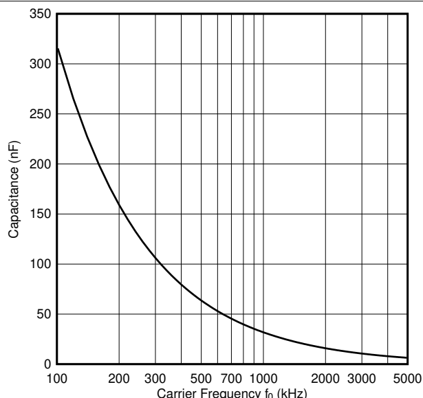
Figure 9-3. Capacitor selection (select values above the line)
