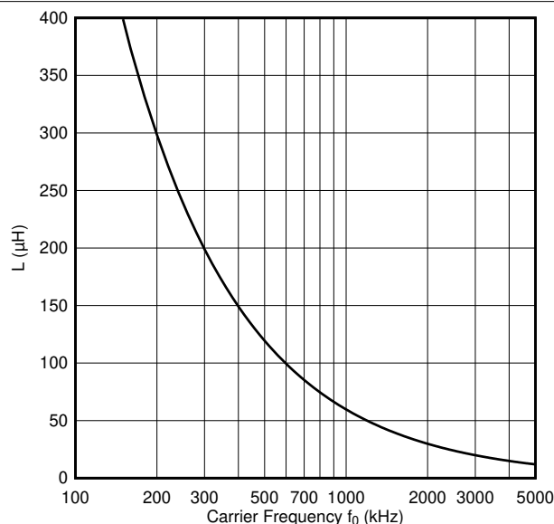
Figure 9-2. Inductor selection (select values above the line)
