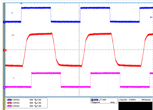
Figure 8-8. THVD2410V Waveforms at V_{CC} = 5 V
