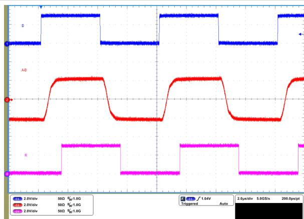
Figure 8-9. THVD2410V Waveforms at V_{CC} = 3.3 V
