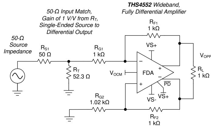
Figure 8-4. Single-Ended to Differential Gain of 1 V/V with Input Matching Using Standard Resistor Values
