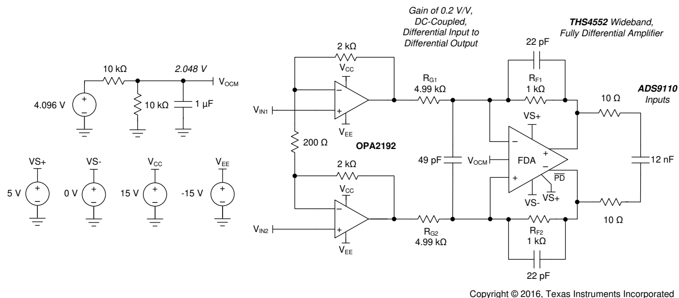
Figure 8-11. Example DC-Coupled Differential I/O Design from a Precision Dual Op Amp to an 18-Bit SAR
