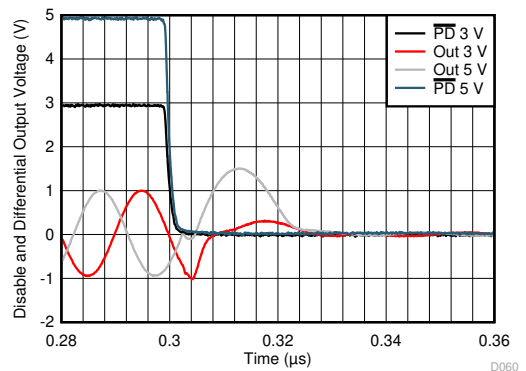
Figure 6-60. \overline{\text{PD}} Turn Off Waveform
