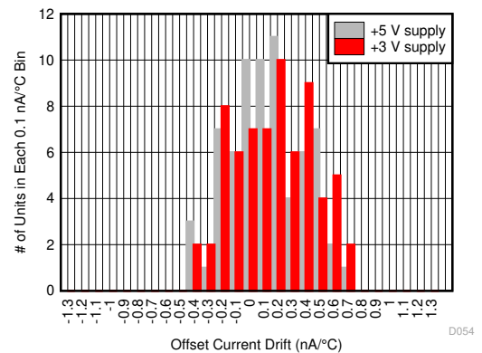
Figure 6-52. Input Offset Current Over Temperature
