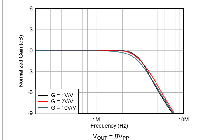
Figure 6-5. Large-Signal Bandwidth vs Gain
