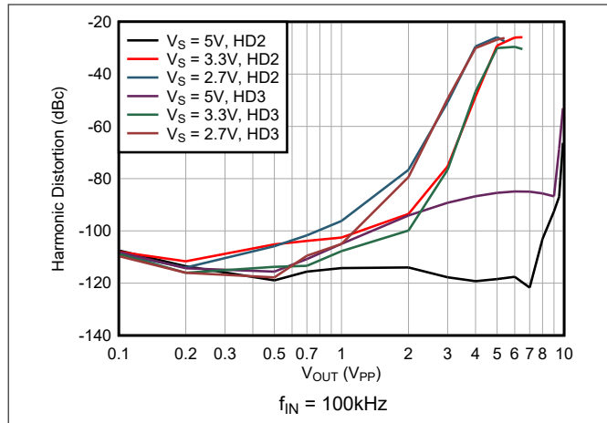
Figure 6-25. Harmonic Distortion vs Output Amplitude
