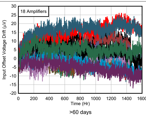
Figure 6-36. THS4536 Long Term Drift
