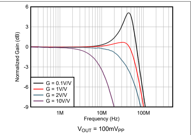
Figure 6-2. Small-Signal Bandwidth vs Gain
