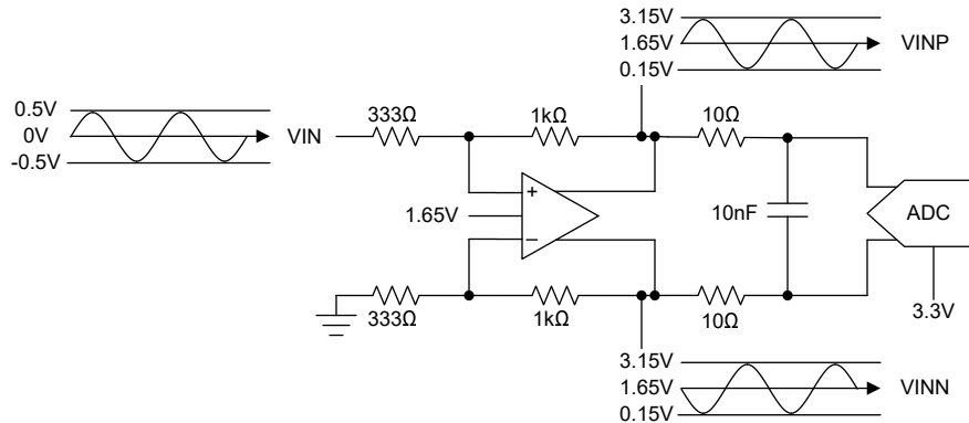
Figure 8-4. THS4536 Single-to-Differential Conversion
