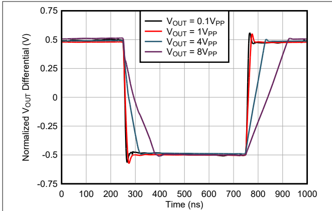
Figure 6-19. Large-Signal Step Response vs Output Amplitude
