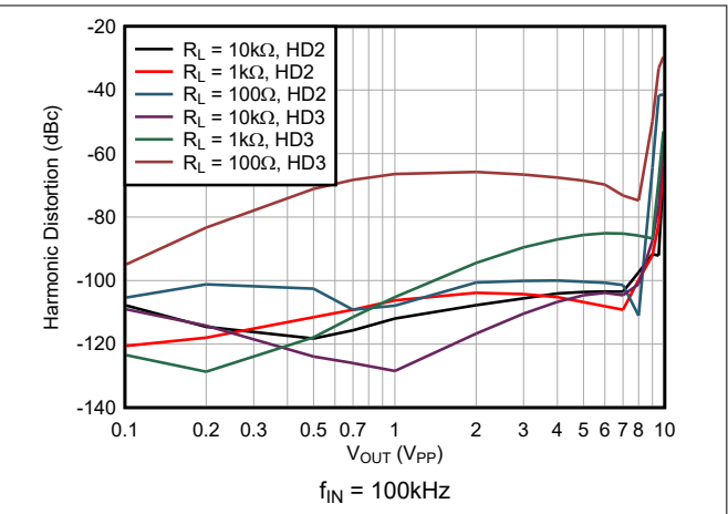
Figure 6-26. Harmonic Distortion vs Output Amplitude
