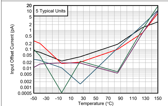
Figure 6-33. Input Offset Current vs Temperature
