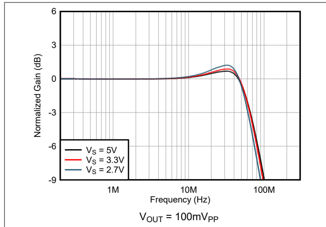
Figure 6-1. Small-Signal Bandwidth vs Supply Voltage
