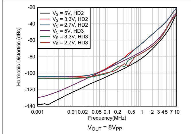
Figure 6-27. Harmonic Distortion vs Frequency
