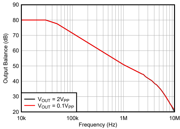
Figure 6-13. Output Balance vs Frequency
