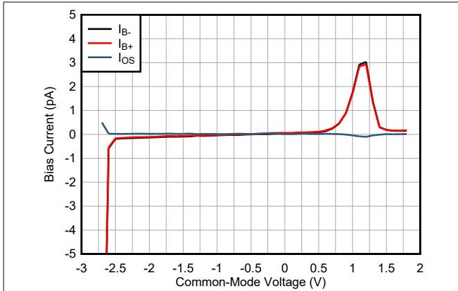
Figure 6-31. Input Bias Current vs Input Common-Mode Voltage
