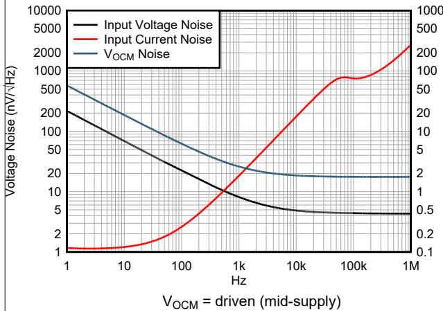
Figure 6-11. Voltage Noise vs Frequency
