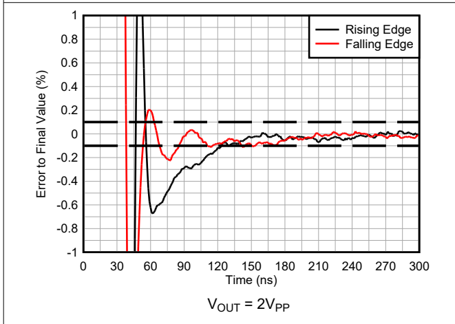
Figure 6-21. Large Signal Settling Time
