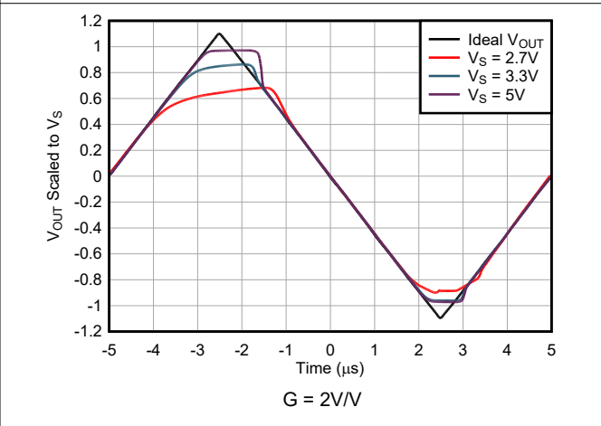
Figure 6-22. Overload Recovery Time vs Supply Voltage
