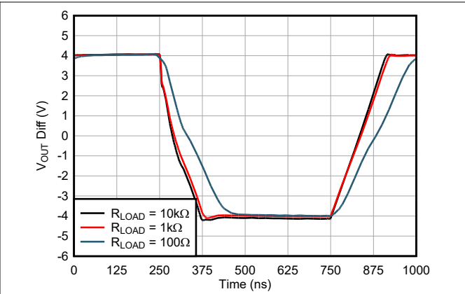
Figure 6-20. Large Signal Step Response vs Resistive Load
