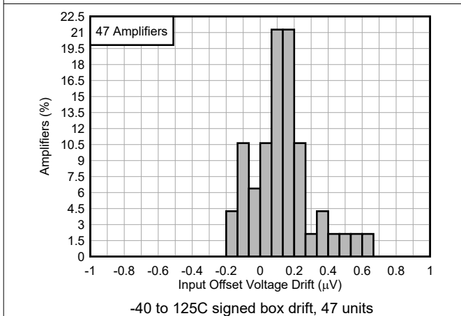
Figure 6-35. THS4536 Offset Voltage Drift Distribution
