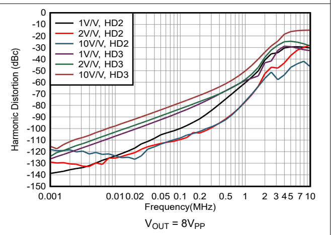
Figure 6-28. Harmonic Distortion vs Frequency
