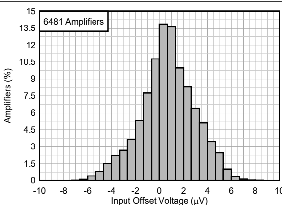
Figure 6-34. THS4536 Offset Voltage Distribution
