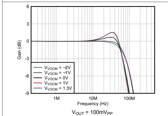
Figure 6-3. Small-Signal Bandwidth vs Output Common-Mode
