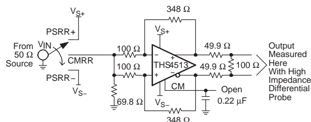
Figure 59. CMRR and PSRR Test Circuit
