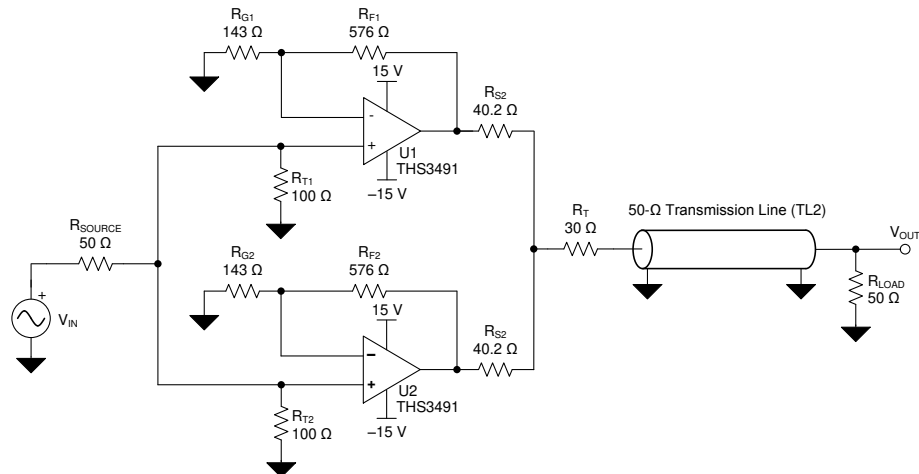
Figure 10-5. Load-Sharing Driver Application
