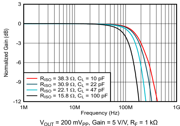
Figure 7-7. Capacitive Load Frequency Response
