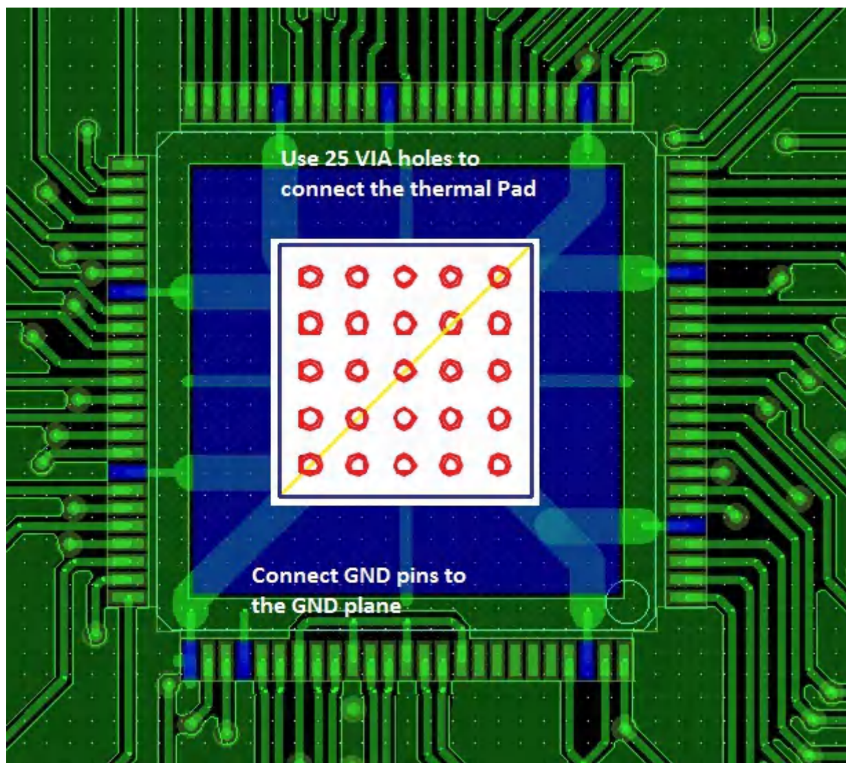
Figure 7-9. Ground Routing
