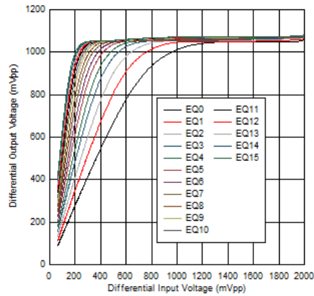
Figure 5-3. DisplayPort Linearity Curves at 4.05GHz
