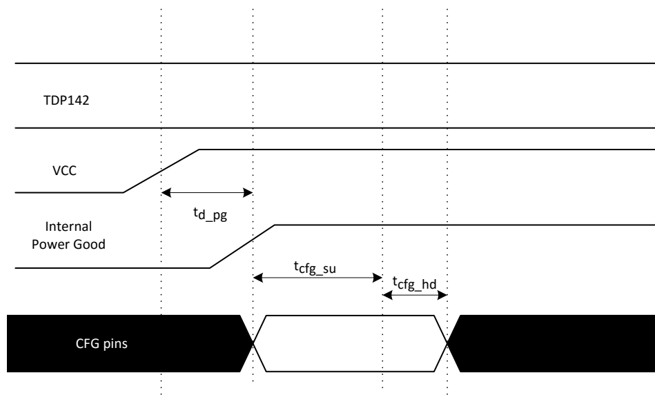
Figure 6-1. Power-Up Timing
