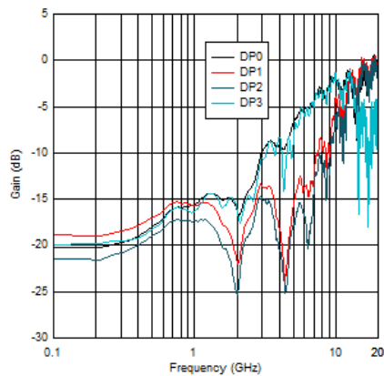
Figure 5-5. DisplayPort Output Return Loss Performance
