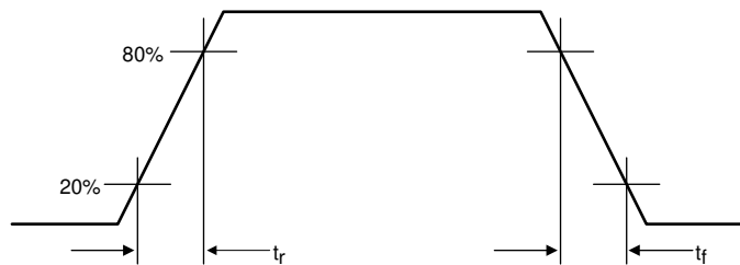
Figure 6-3. Output Rise and Fall Times
