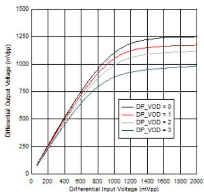
Figure 5-7. DP VOD Linearity Settings at 100MHz
