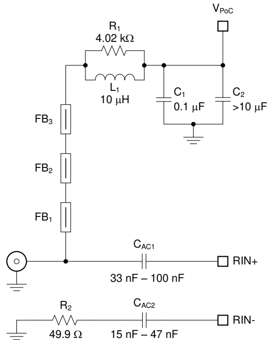
Figure 8-2. Example Recommended PoC Network for a "4G" V³Link
