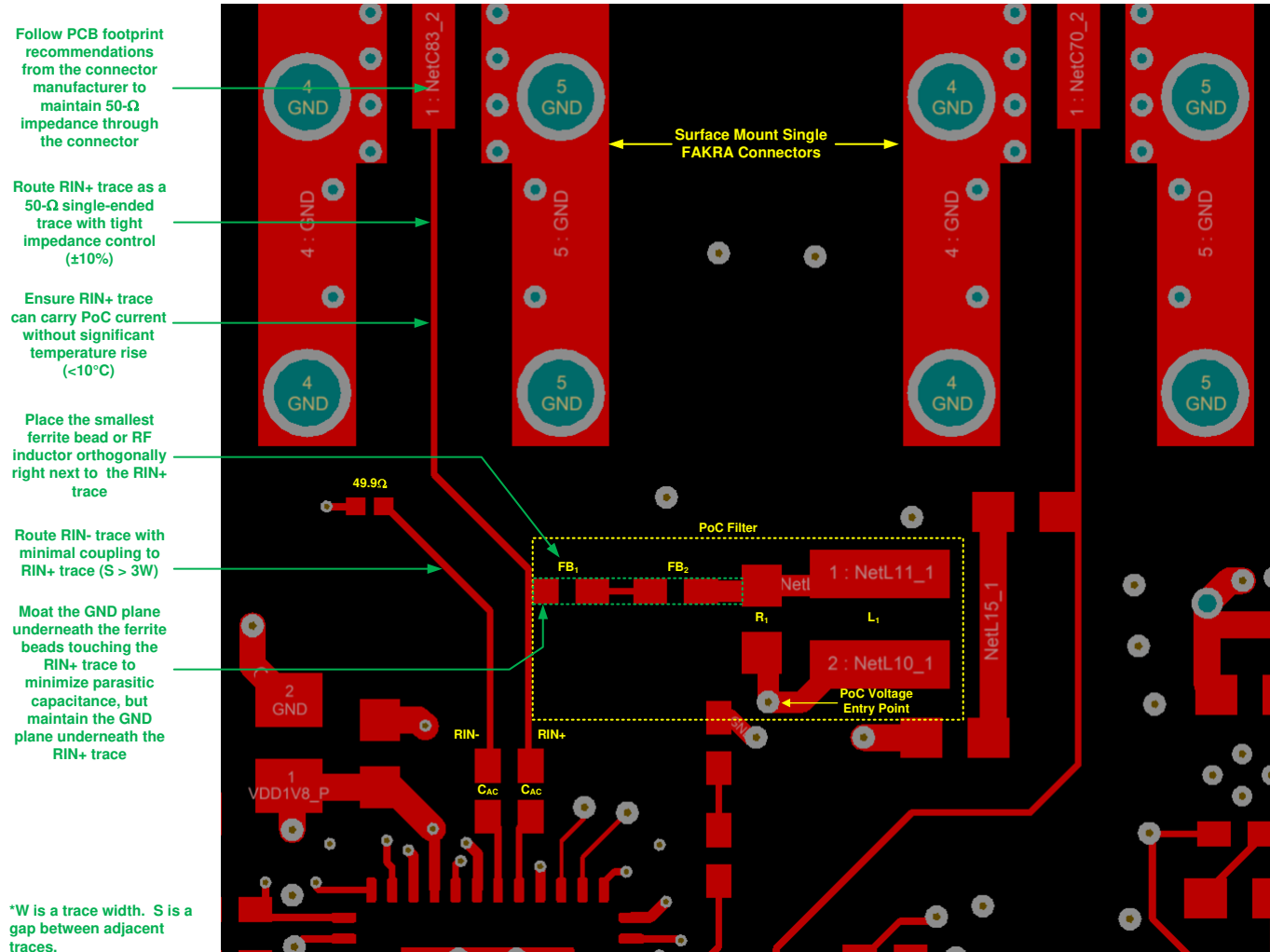
Figure 8-22. Example Routing of V³Link Traces to a Single Mini-Fakra Connector and PoC Components
