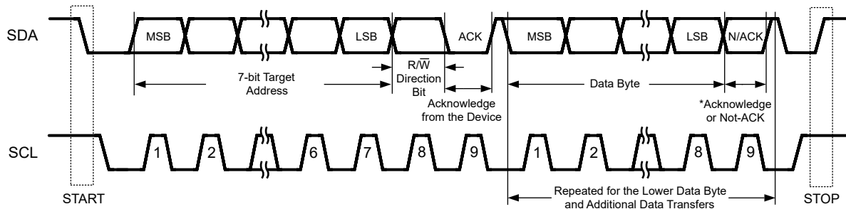
Figure 7-25. Basic Operation
