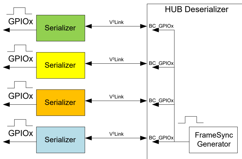
Figure 7-16. Internal FrameSync
