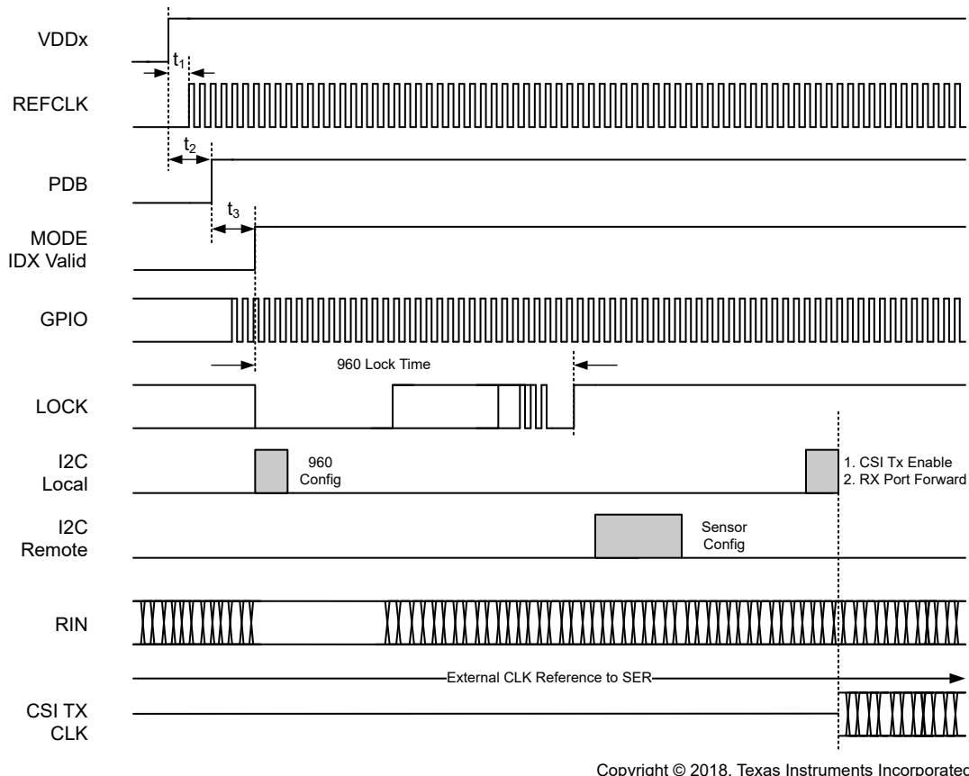
Figure 8-20. Power-Up Sequencing With Non-Synchronous Clocking Mode
