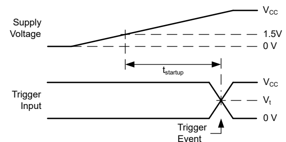
Figure 6-6. Voltage Waveforms, Startup Time
