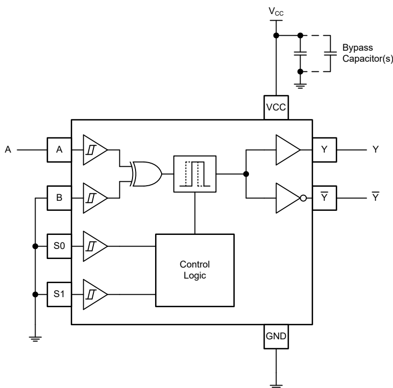
Figure 8-1. Delay Schematic Using the TDEL1G522-Q1
