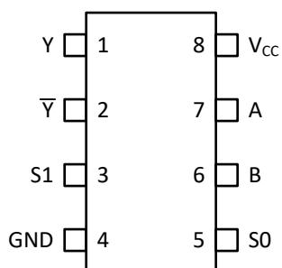
Figure 4-1. TDEL1G522-Q1 DRL Package (Top View)
