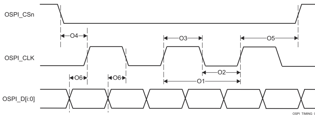
Figure 6-105. OSPI0/1 Switching Characteristics – Tap DDR, No Loopback
