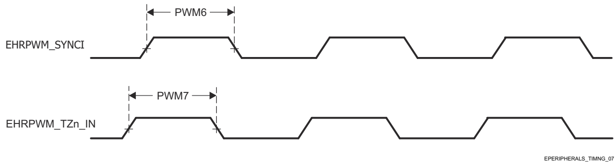
Figure 6-61. ePWM_SYNCI and ePWM_TZn_IN Output Timings
