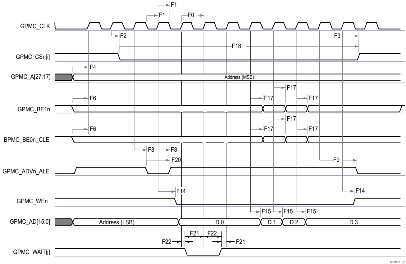
Figure 6-55. GPMC and Multiplexed NOR Flash — Synchronous Burst Write
