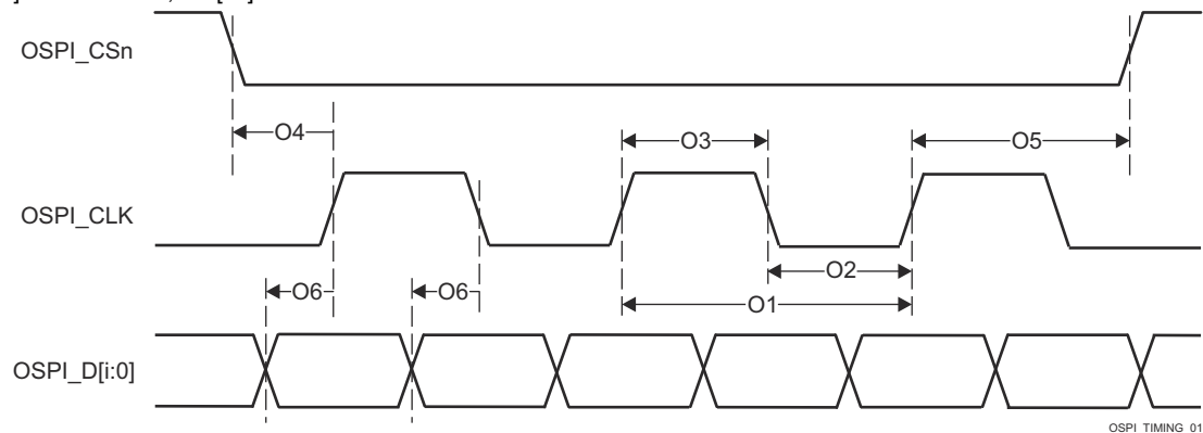
Figure 6-106. OSPI Switching Characteristics – DDR
