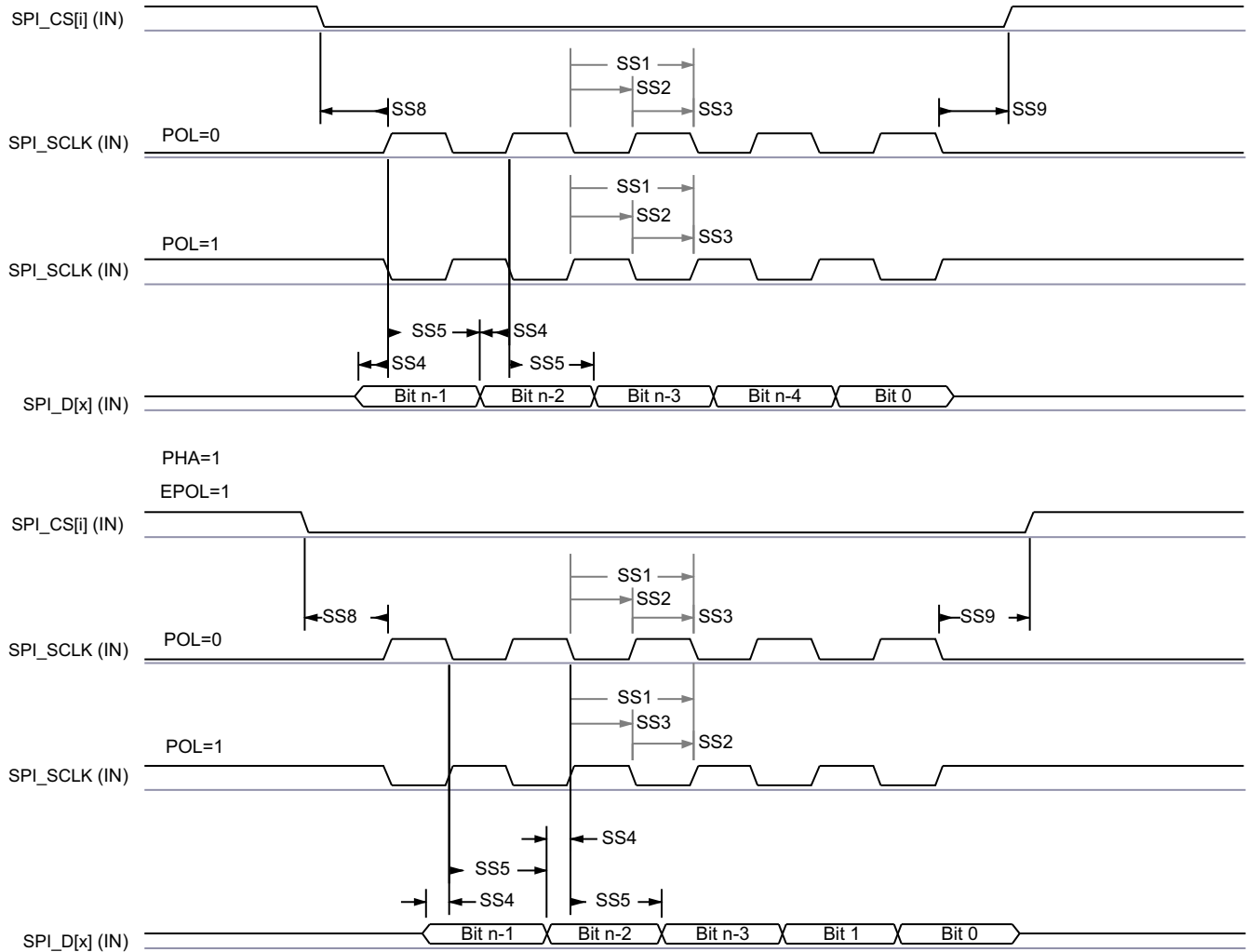
Figure 6-75. SPI Peripheral Mode Receive Timing
