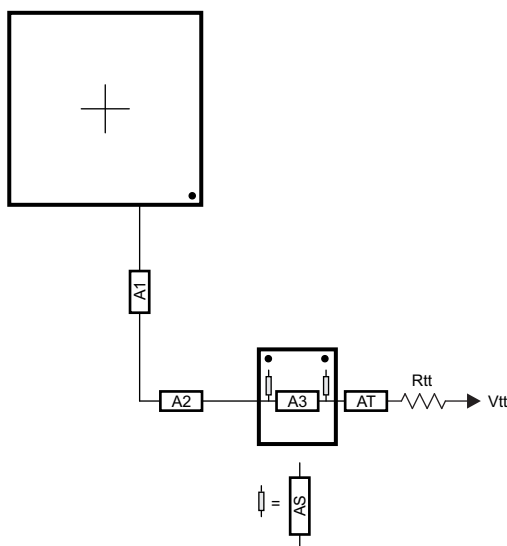
Figure 8-59. CK Routing for Two Mirrored DDR3 Devices
