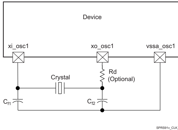
Figure 6-6. Crystal Implementation
