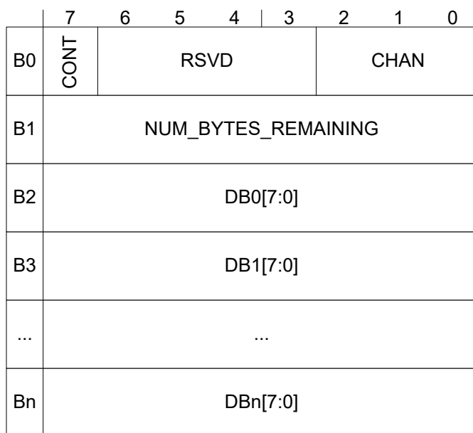
Figure 7-81. SPI Receive FIFO
