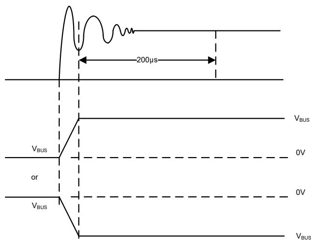
Figure 7-8. Driver Short-Circuit Current Test and Measurement
