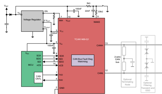
Simplified Schematics
