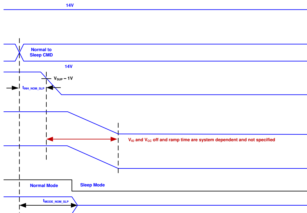
Figure 7-14. Normal to Sleep Timing
