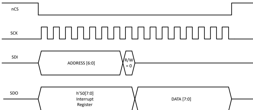
Figure 8-43. SPI Read
