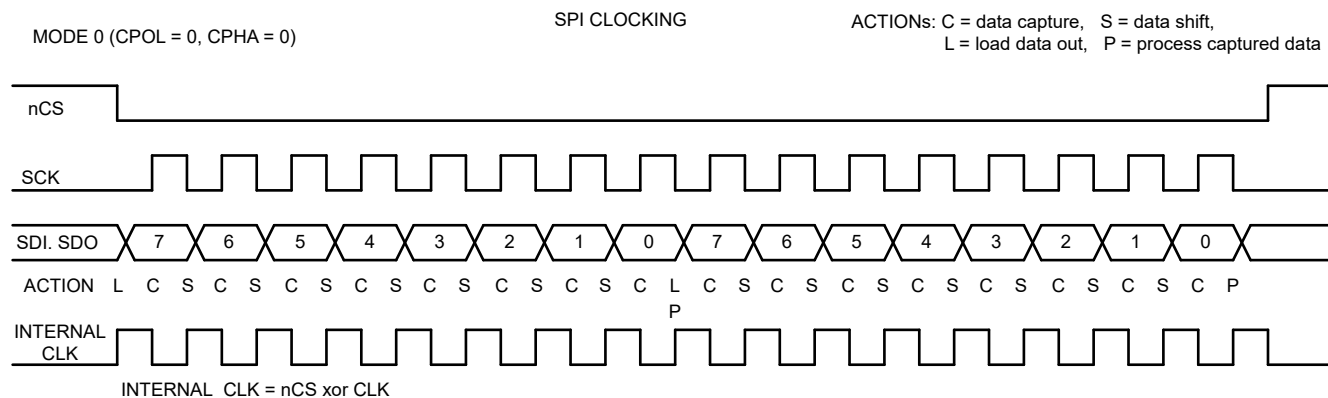
Figure 8-40. SPI Clocking
