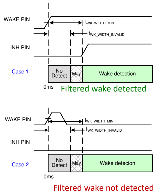
Figure 8-18. WAKE Pin Filtered Behavior
