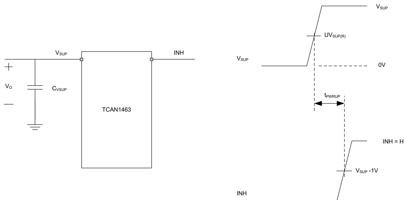
Figure 8-12. Power-Up Timing
