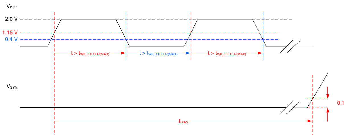
Figure 8-9. Bias Reaction Time Measurement
