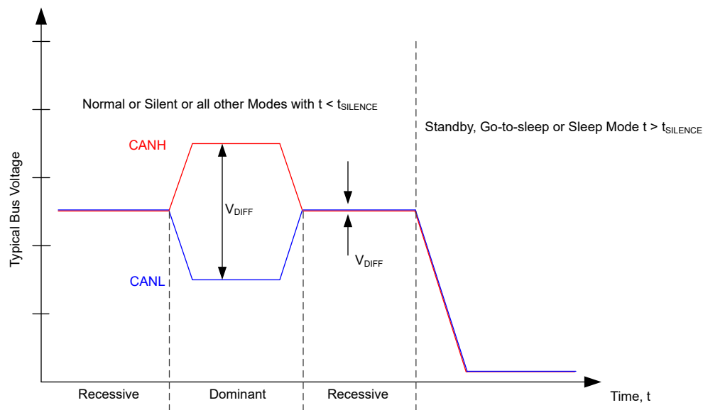
Figure 9-13. Bus States
