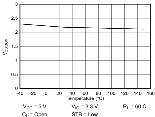
Figure 6-1. V_{OD(DOM)} Overtemperature
