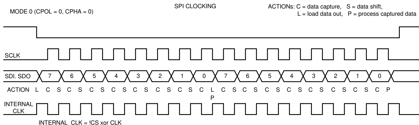
Figure 9-21. SPI Clocking
