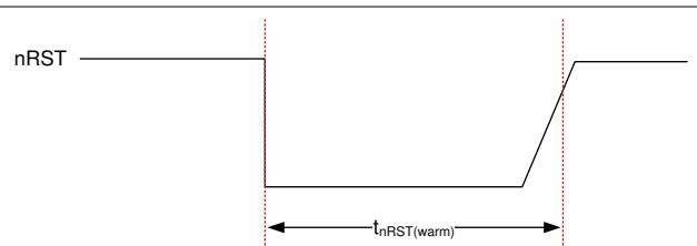
Figure 8-5. t_{nRST} Warm Start
