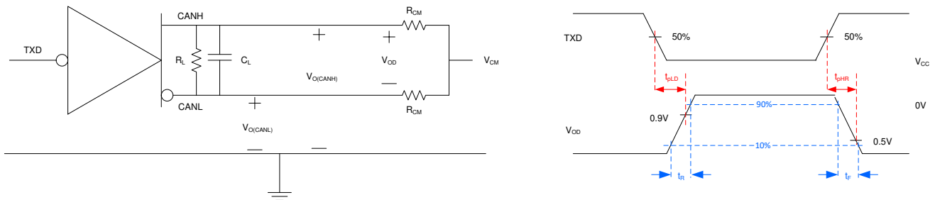
Figure 8-2. Driver Test Circuit and Measurement
