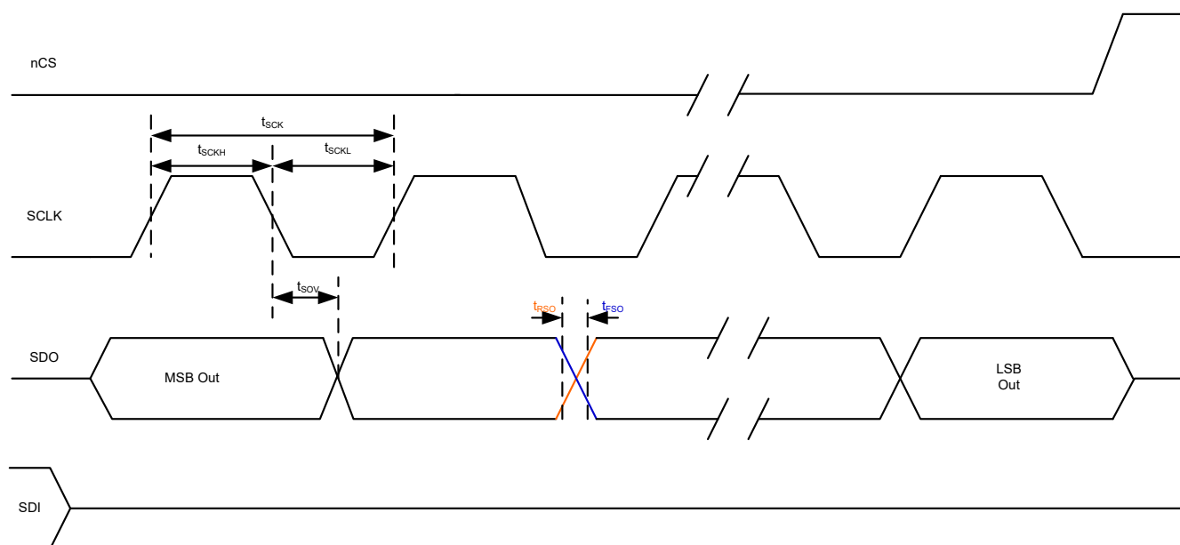
Figure 8-13. SPI AC Characteristic Read
