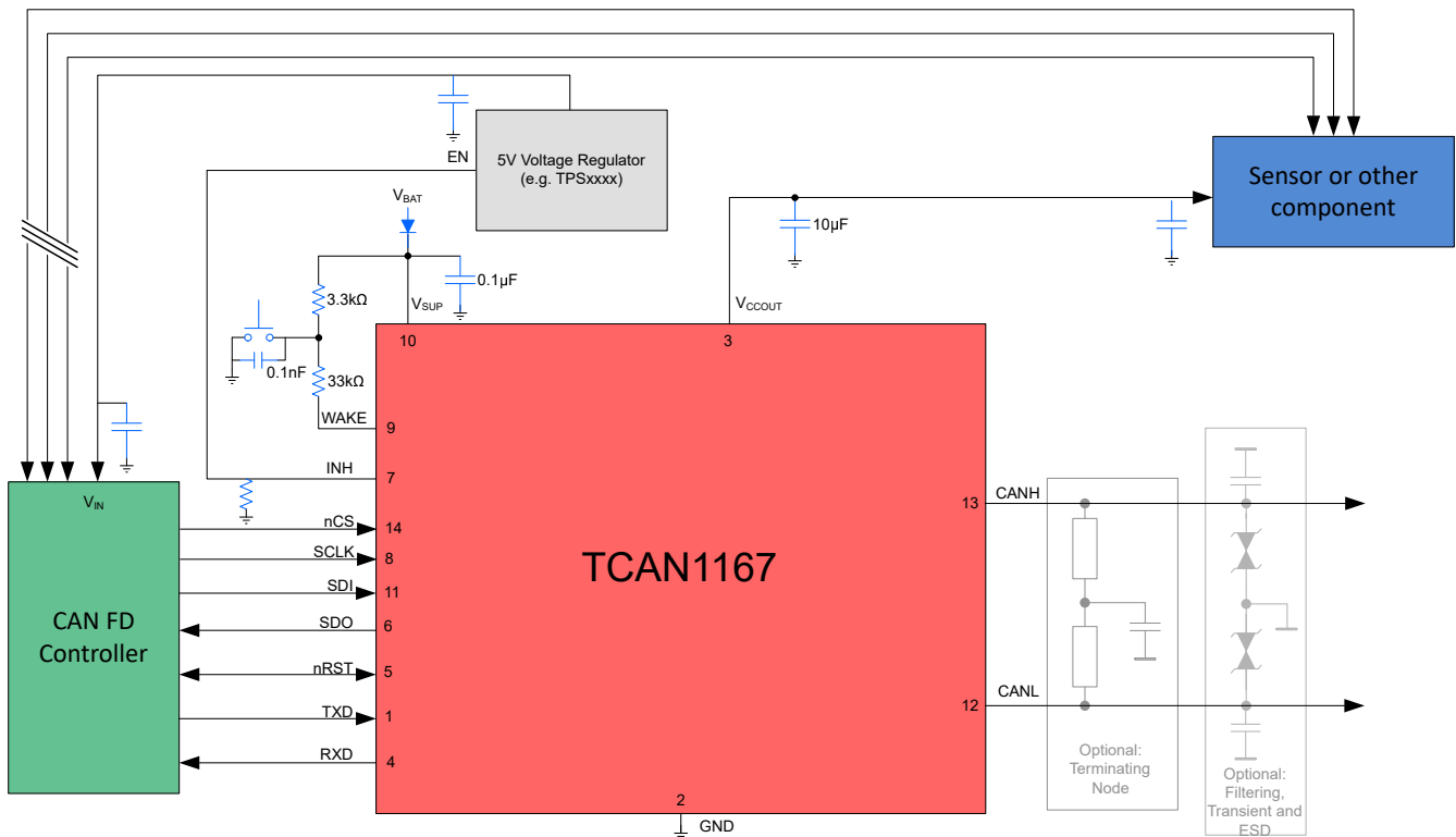
Figure 10-1. Typical Application
