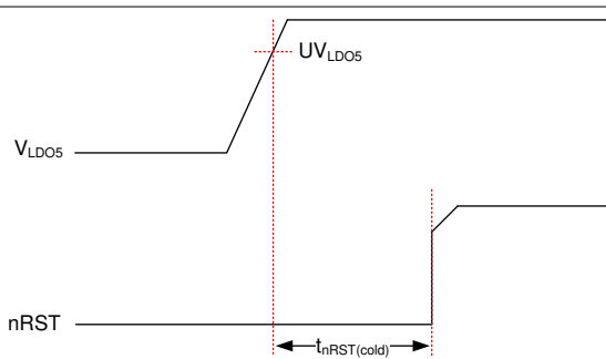
Figure 8-4. t_{nRST} Cold Start
