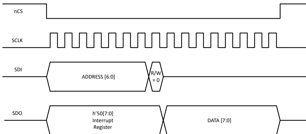
Figure 9-24. SPI Read
