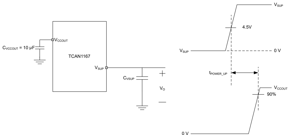
Figure 8-9. t_{\text{POWER\_UP}} Timing Measurement
