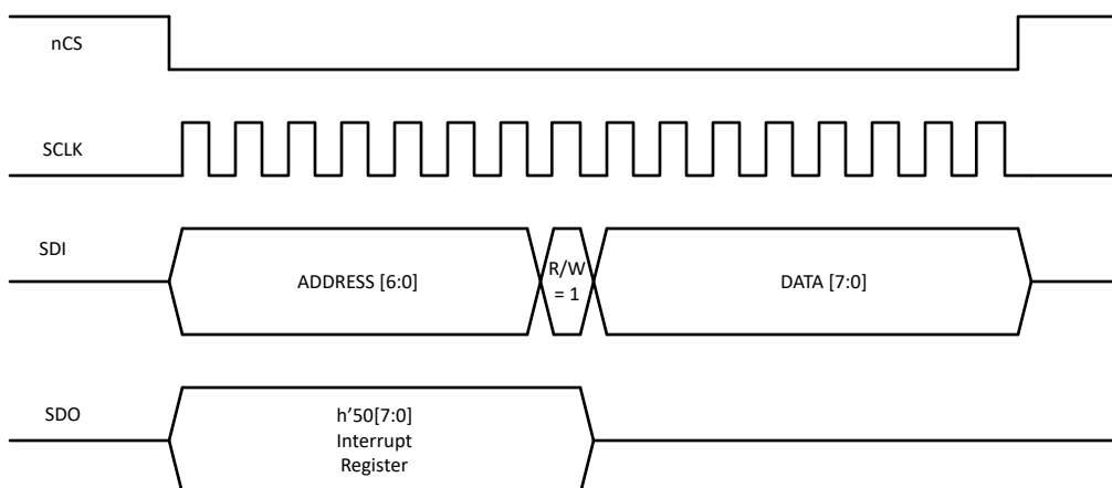
Figure 9-22. SPI Write
