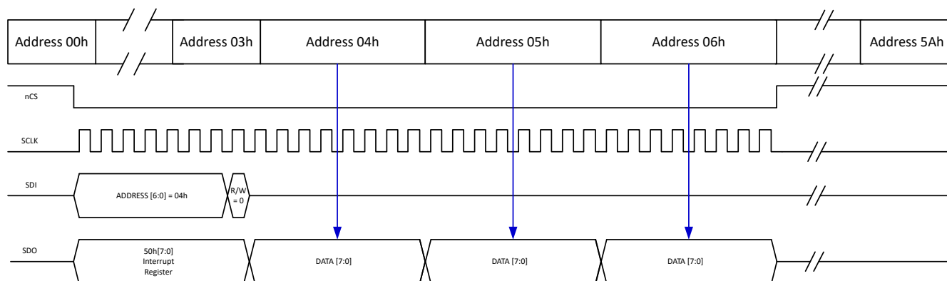
Figure 9-25. 32-bit SPI Burst Read
