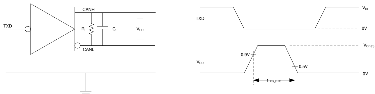
Figure 6-5. TXD Dominant Timeout Test Circuit and Measurement
