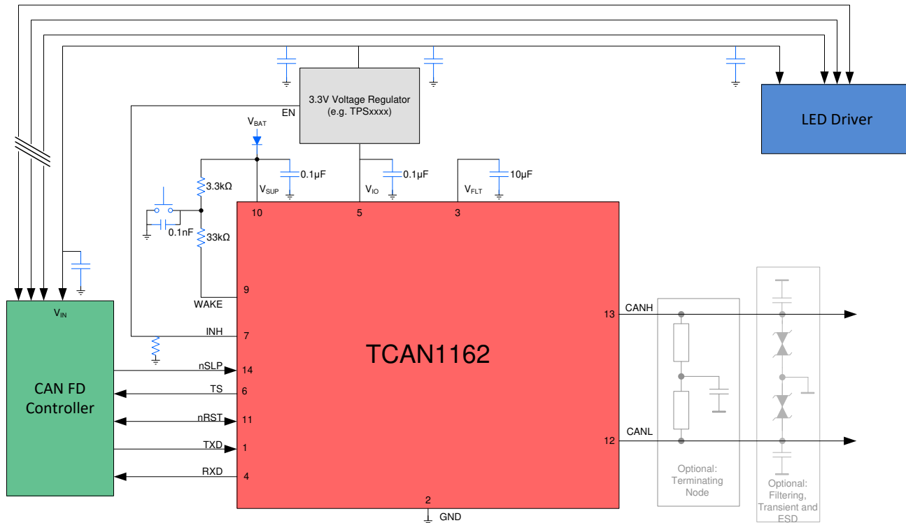
Simplified Schematic
