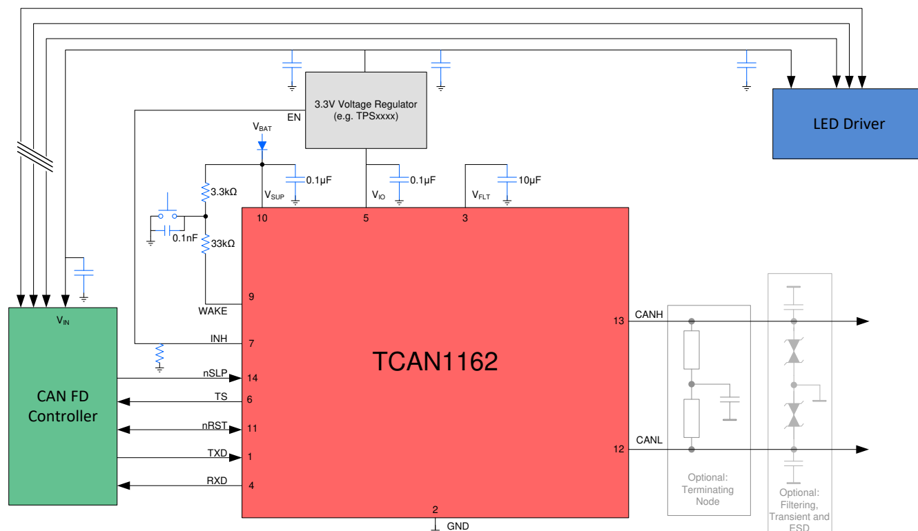
Figure 8-1. Typical Application
