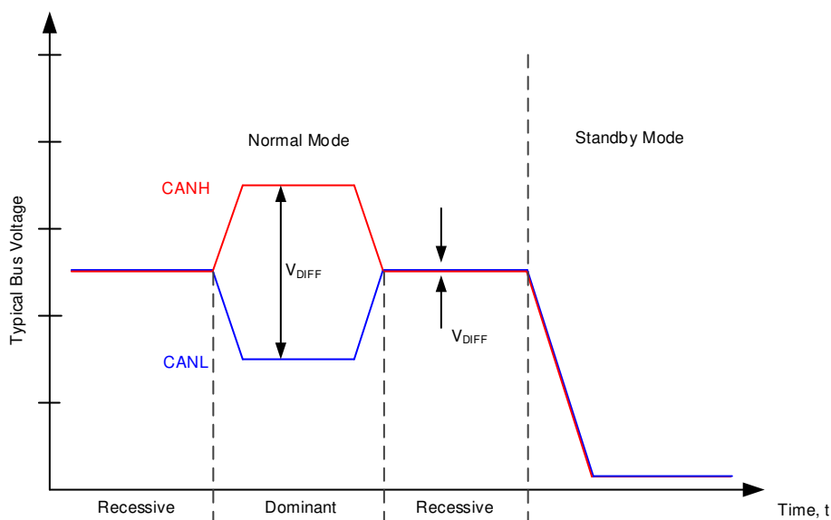
Figure 7-9. Bus States
