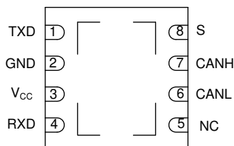
Figure 5-2. DRB Package for Base, (H), (G), and (HG) Devices 8 PIN (VSON) Top View
