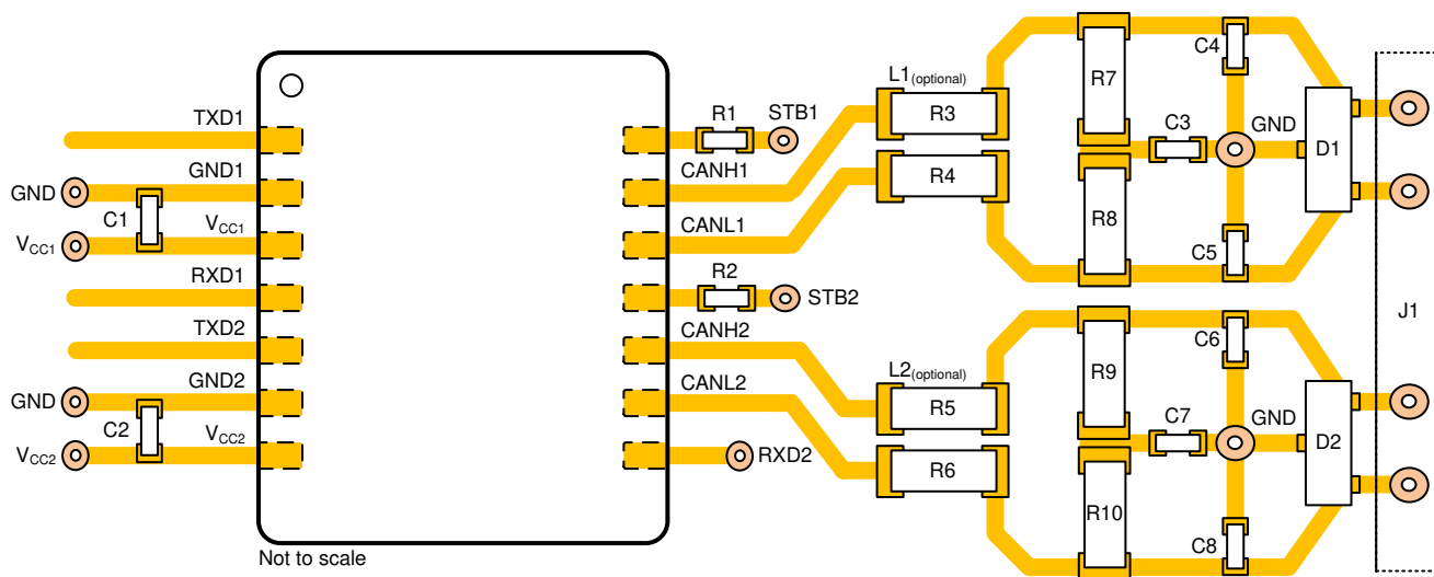
Figure 11-1. Layout Example
