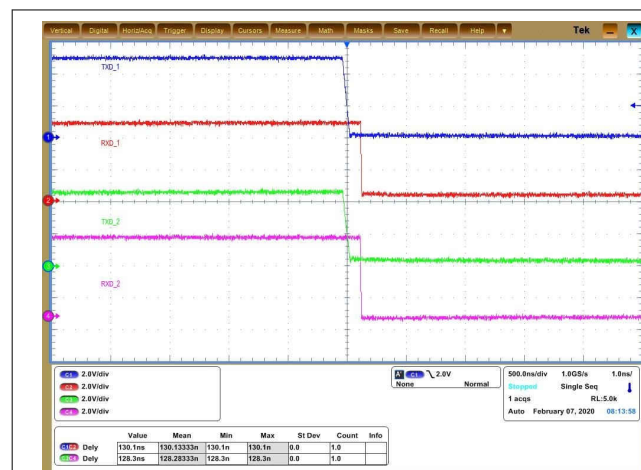
Figure 9-4. t_{\text{PROP(LOOP1)}} Transceiver 1 & Transceiver 2
