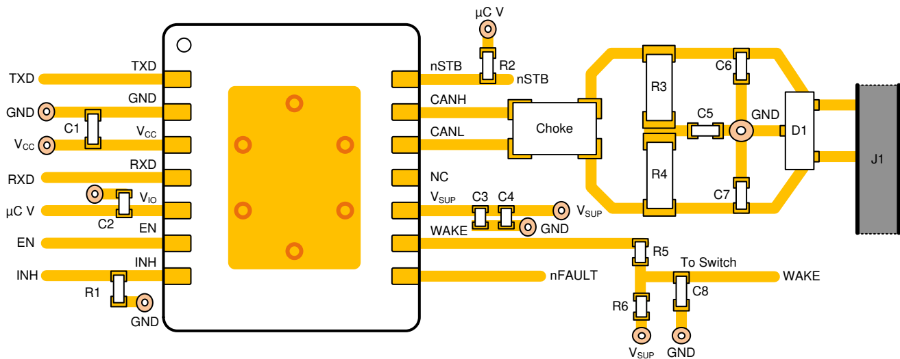
Figure 8-4. Example Layout
