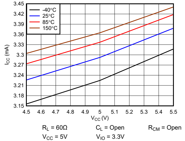
Figure 5-2. I_{CC} Recessive vs V_{CC} and Temperature
